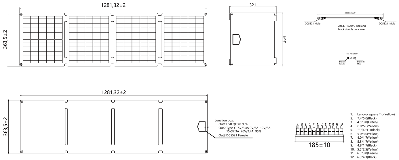
BXF-N-4*15W
