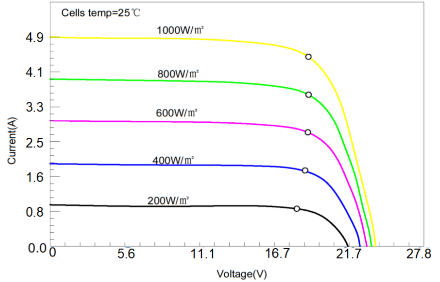
SGF-FL-90W
